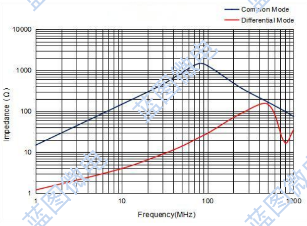
SMDCM5020-142T&152T
