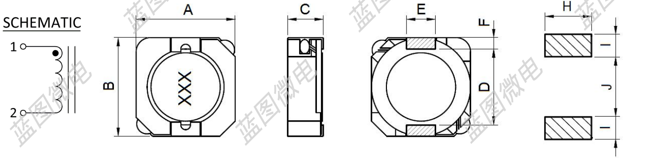
Recommended Land Pattern
