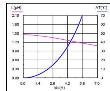
SMS0420-1R5M
