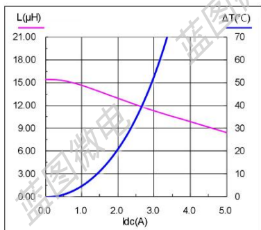
SMS0530-150M
