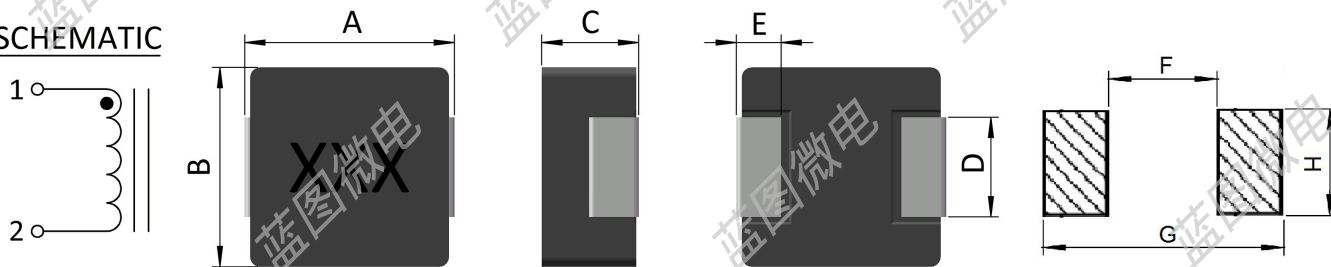
Land Pattern
