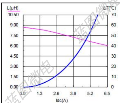
SMS0630-8R2M
