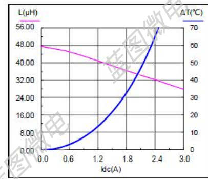
SMS0630-470M
