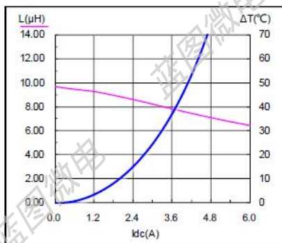
SMS0630-100M
