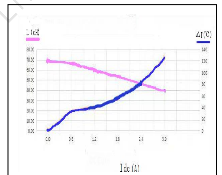
SMS0630-680M
