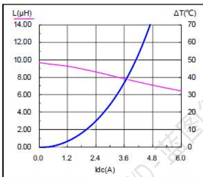
SMS0630-100M
