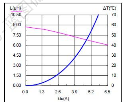
SMS0630-8R2M
