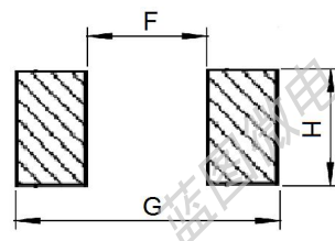
Land Pattern
