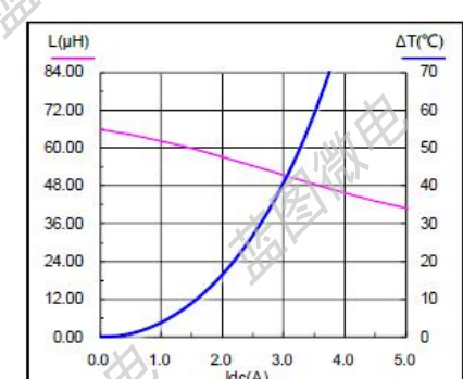
SMS1040-680M
