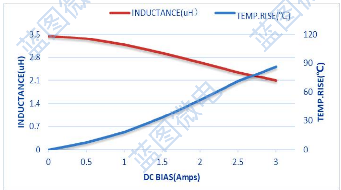
STC201610-3R3M
