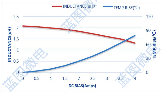
STC201610-2R2M
