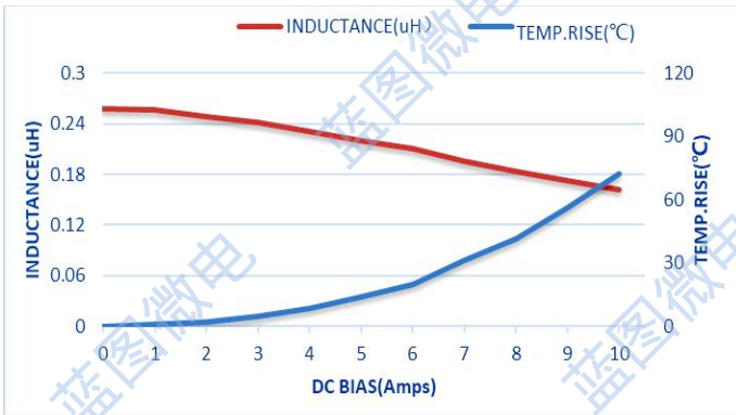
STC201610-R22M
