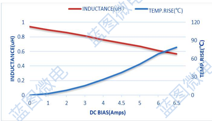
STC201610-1R0M
