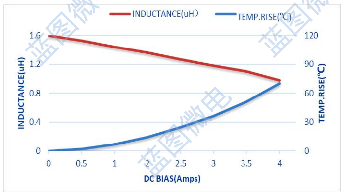
STC201610-1R5M
