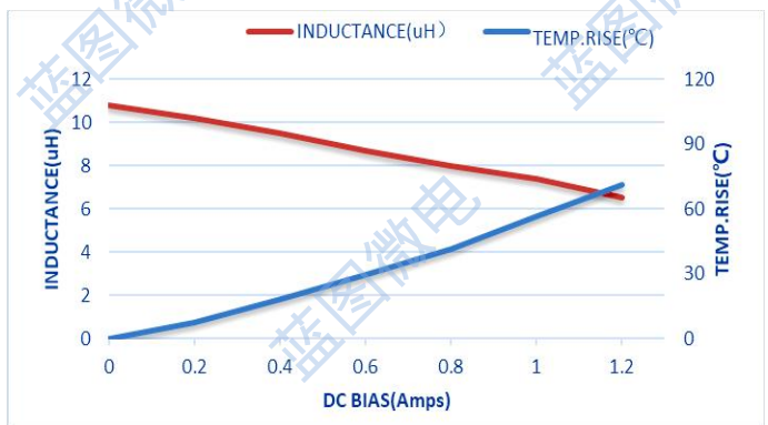
STC201610-100M
