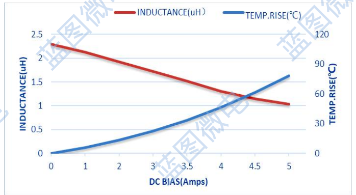
STC201612-2R2M
