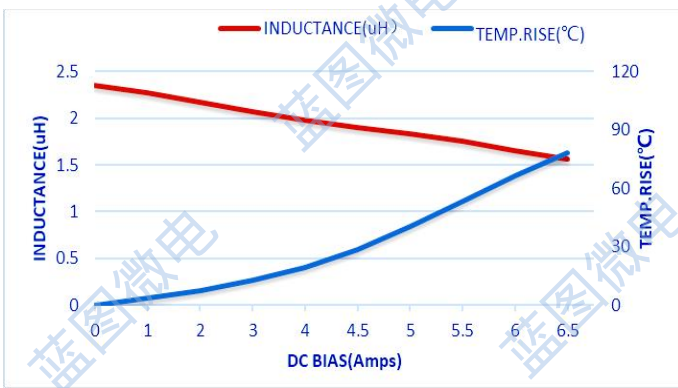
STC303020-2R2M
