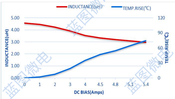
STC303020-4R7M
