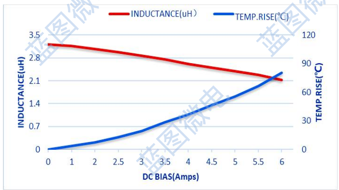
STC303020-3R3M
