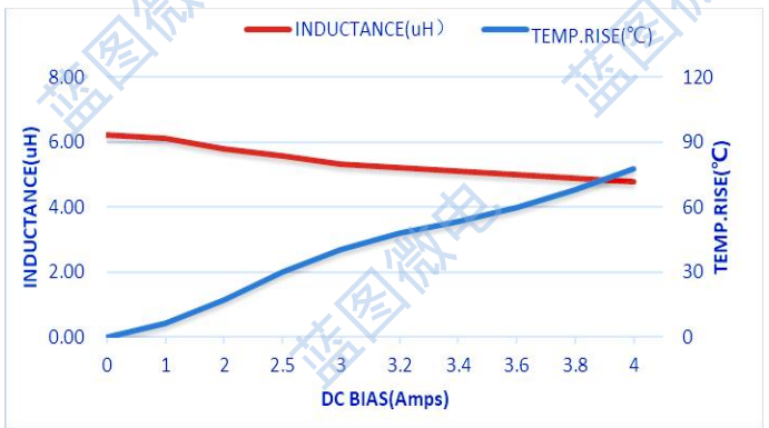
STC303020-6R8M
