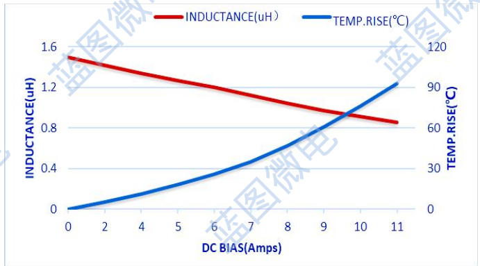
STC303020-1R5M
