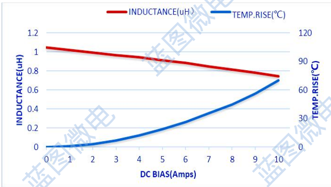
STC303020-1R0M
