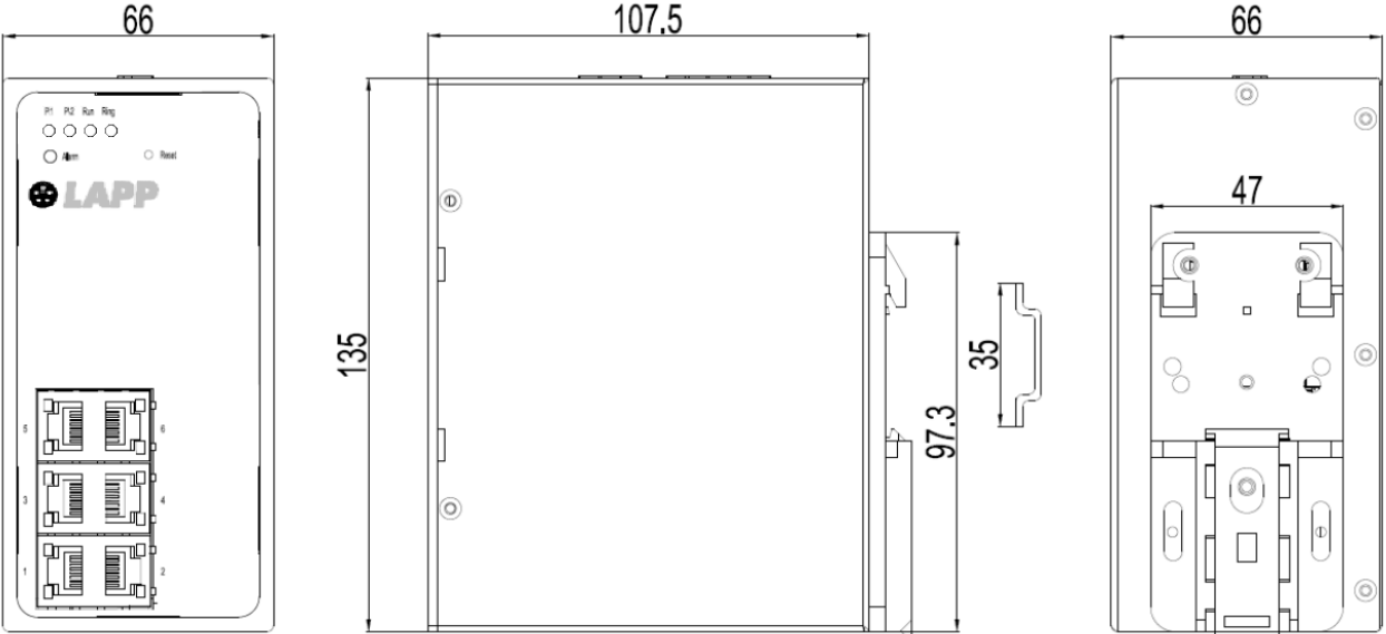
Dimensional drawing (M06T-2GEN)
