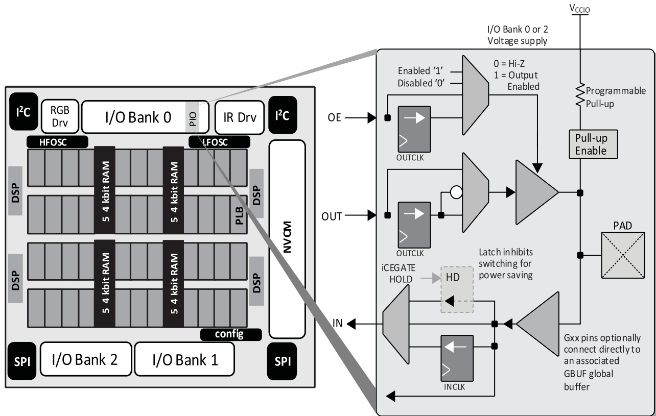
Figure 3.8. I/O Bank and Programmable I/O Cell
