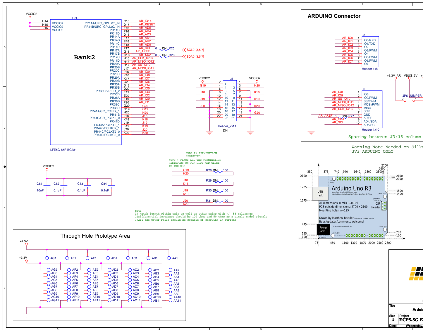
Figure A. 4 Arduino Header (BANK2)
