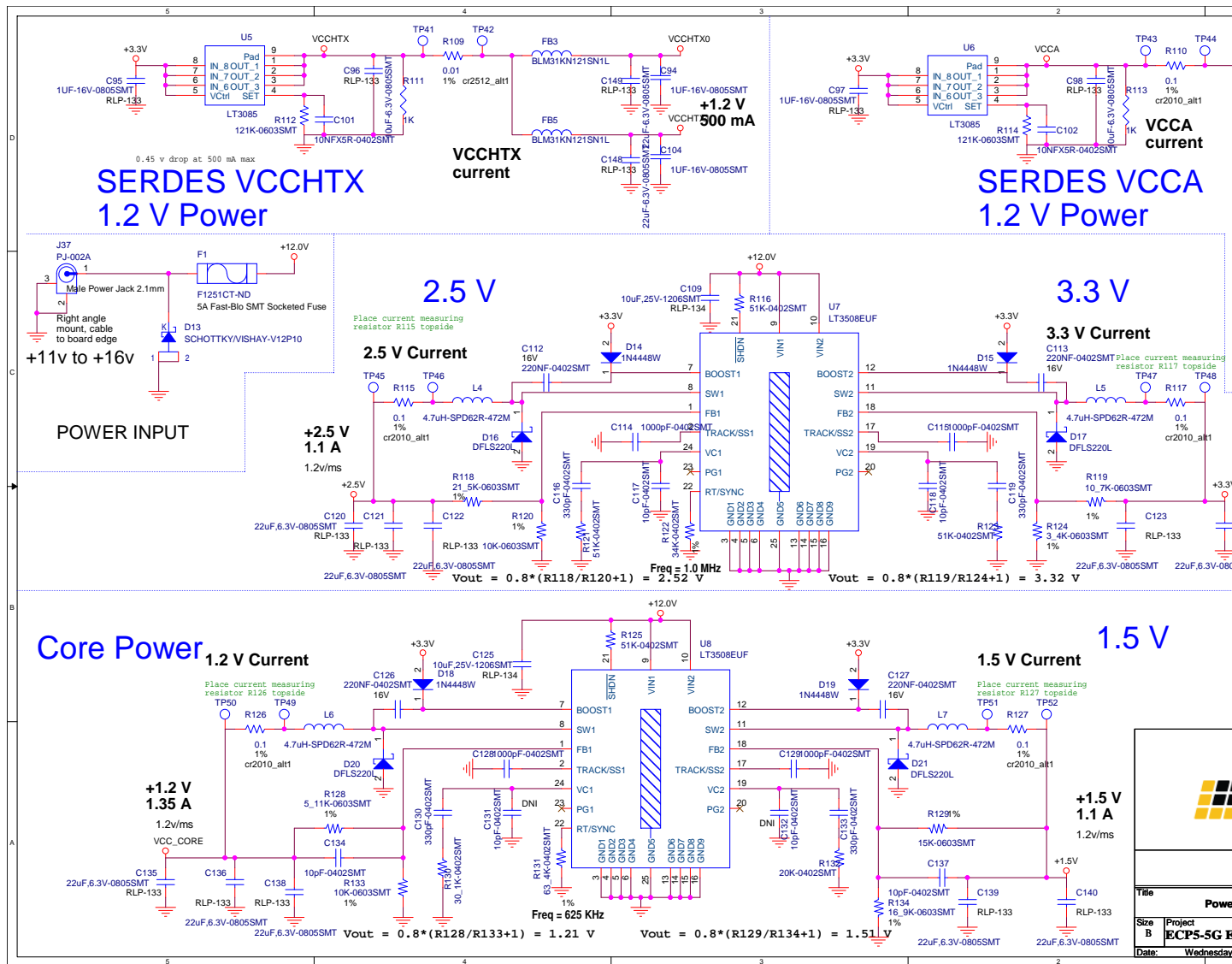
Figure A. 12. Power Regulators
