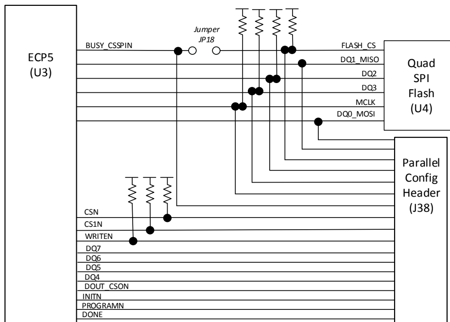
Figure 6.2. SPI Interface
