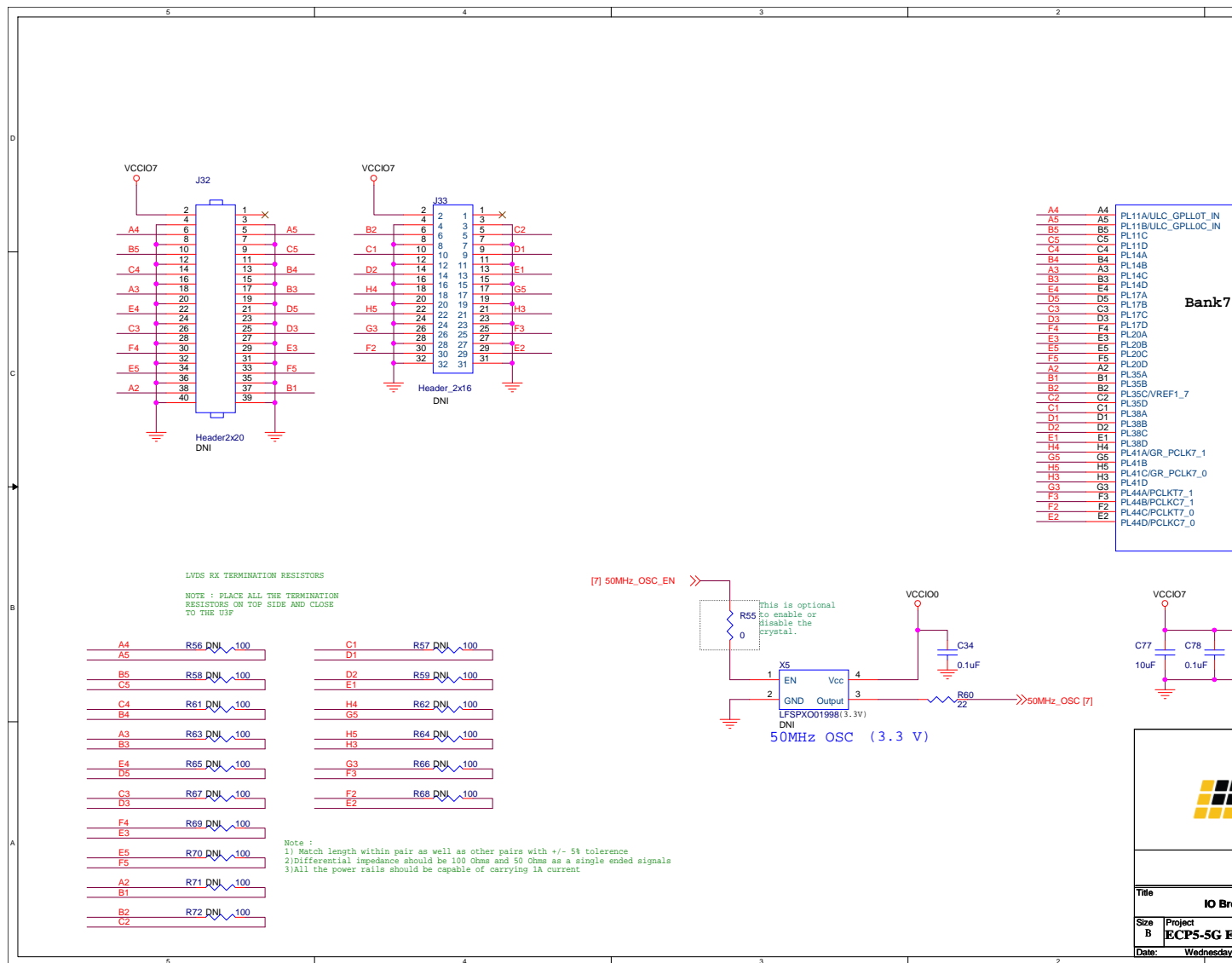
Figure A. 8. IO Breakout (BANK7, Differential Pairs)
