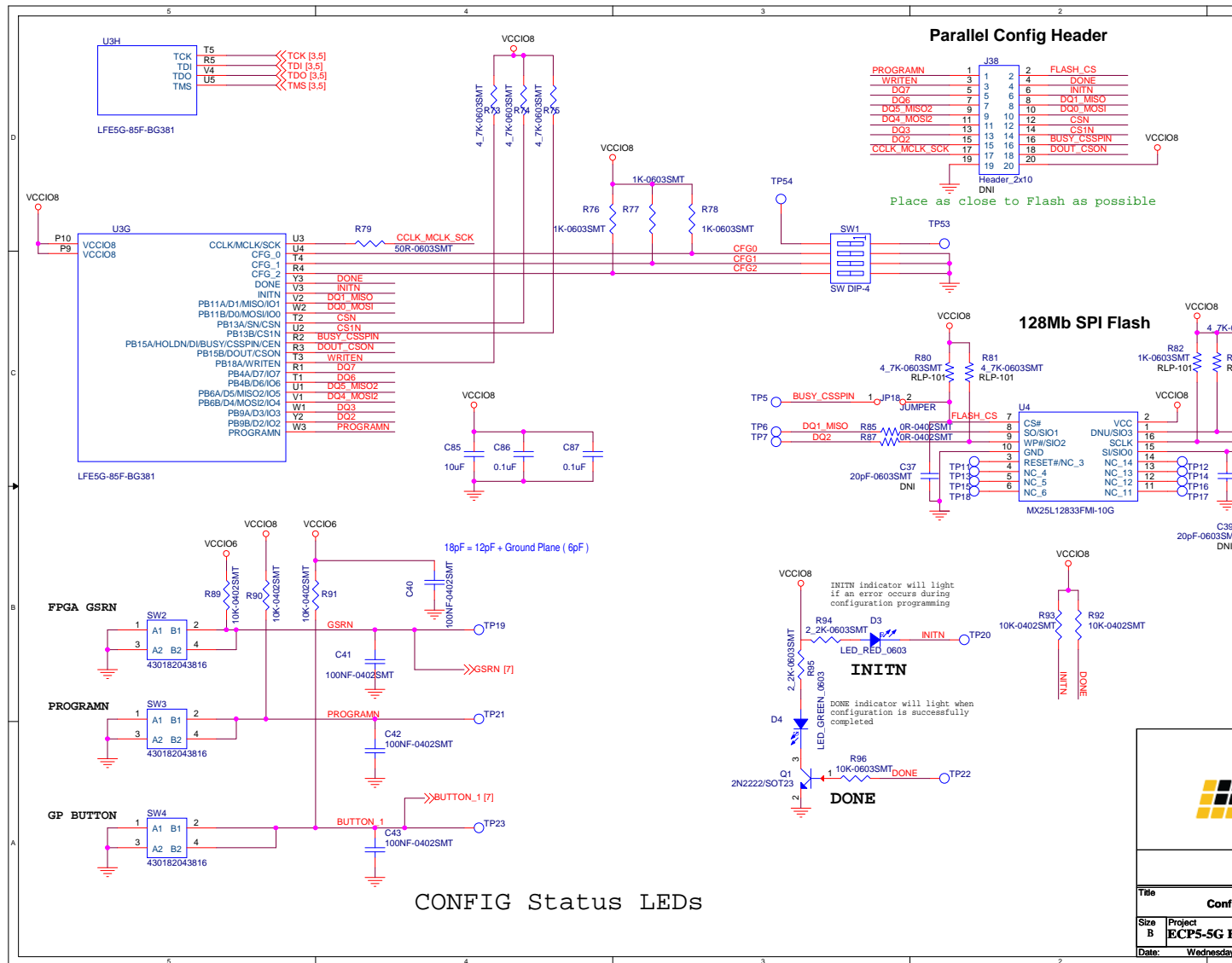
Figure A. 9. Configuration
