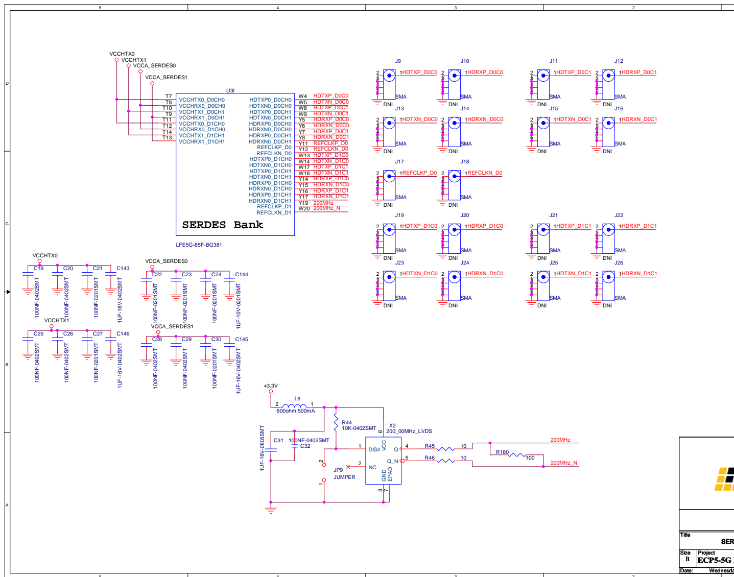
Figure A. 6. SERDES SMA
