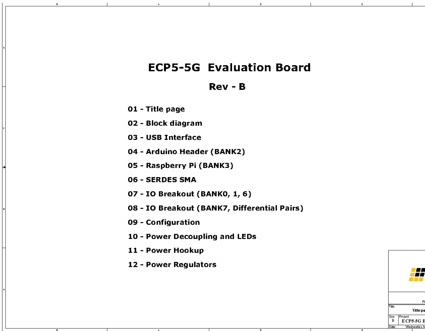
Figure A. 1. Title Page
