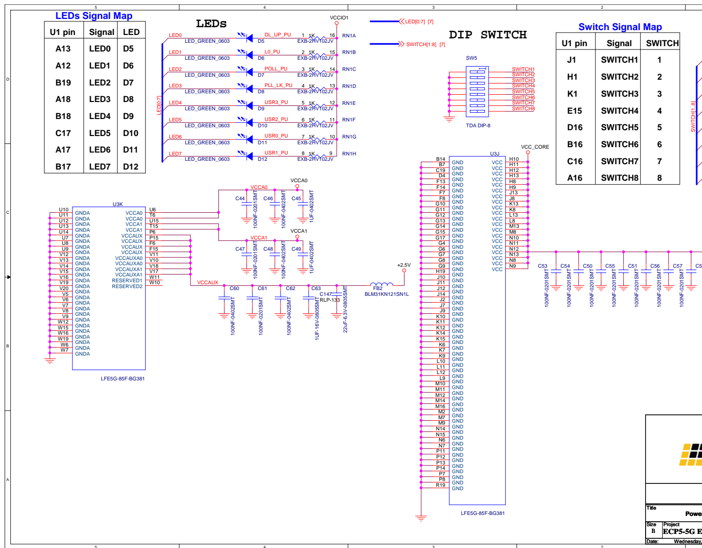
Figure A. 10. Power Decoupling and LEDs
