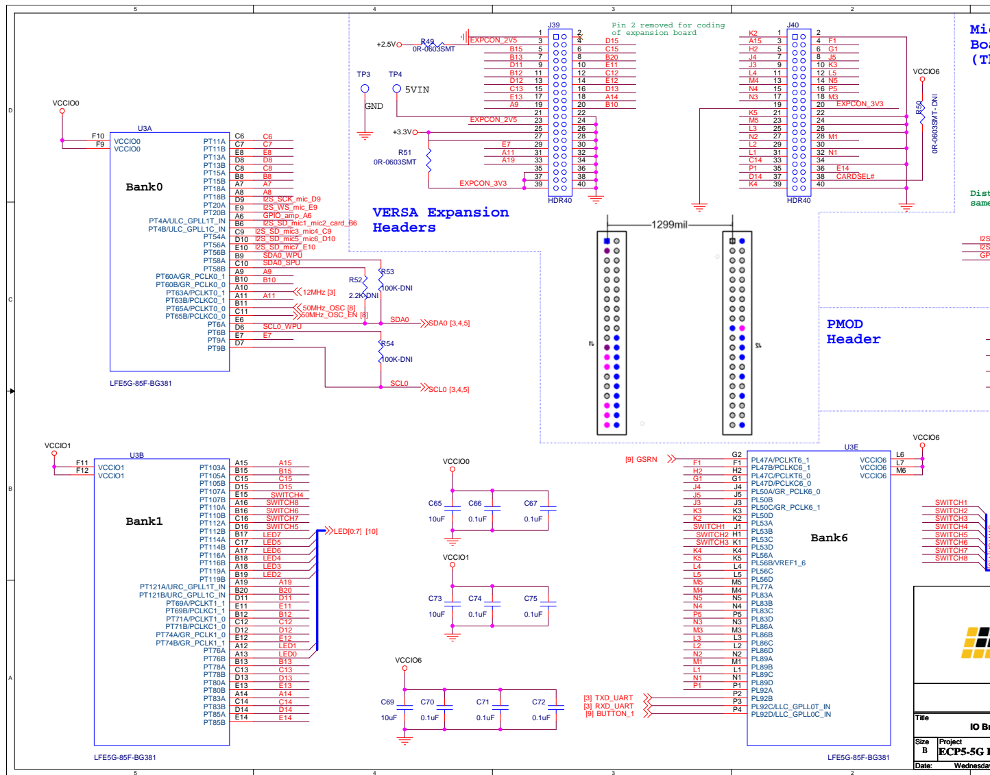
Figure A. 7. IO Breakout (BANK0, BANK1, BANK6)
