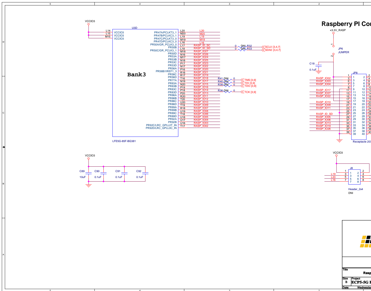
Figure A. 5. Raspberry Pi Header (BANK3)
