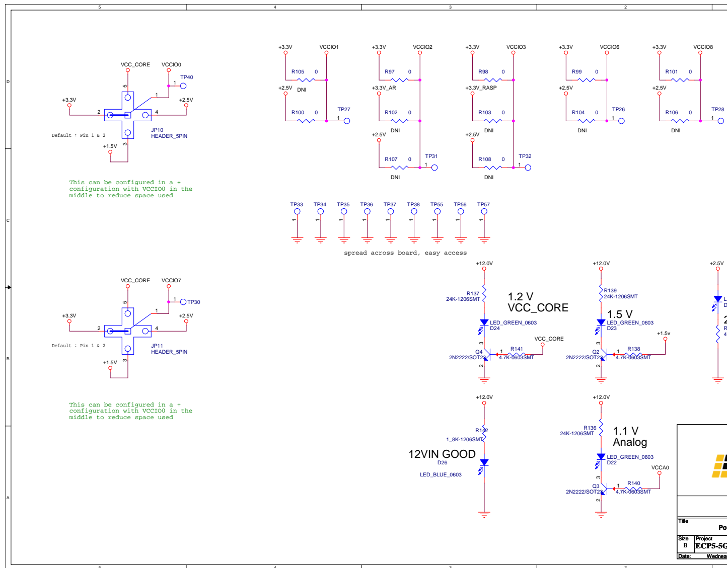
Figure A. 11. Power Hookup
