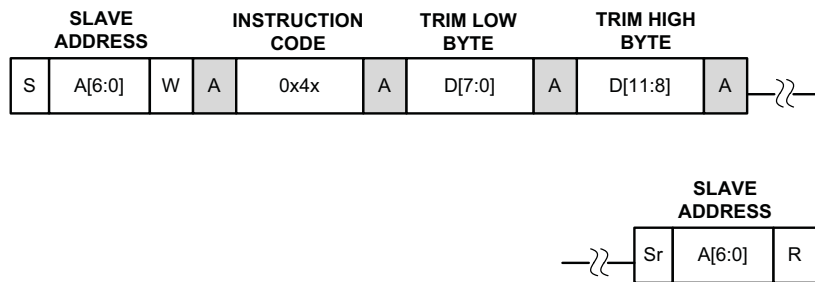
Figure 54. TRIMx_CLT_P0_SET - I 2 C Instruction Format
