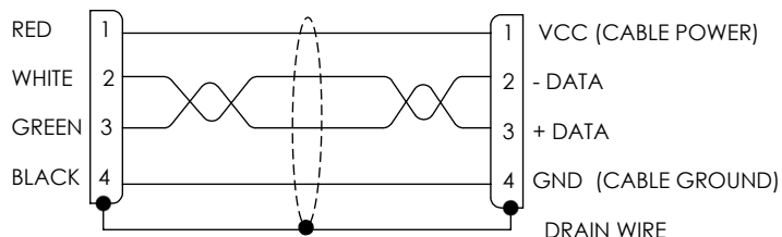
"J1" WIRING DIAGRAM "P1"
