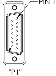
"P1" MALE 15 PIN D-SUB CONNECTOR
