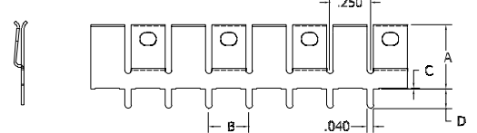
FIGURE 6 .25" Pin Spacing, With Standoff
