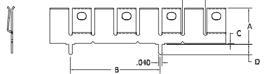
FIGURE 5 .25" Pin Spacing, No Standoff
