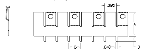
FIGURE 6 .25" Pin Spacing, No Standoff
