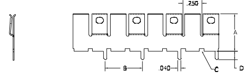
FIGURE 2 .50" Pin Spacing
