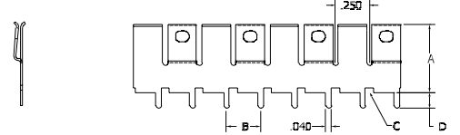
FIGURE 3 .25" Pin Spacing
