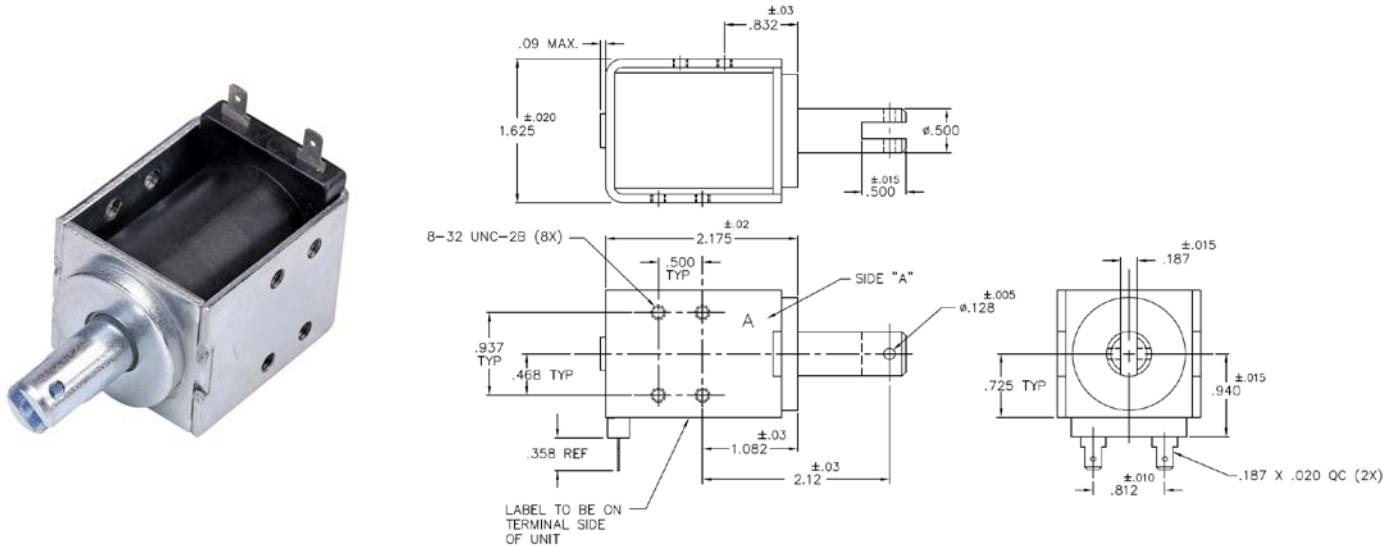
Solenoid shown energized with plunger fully seated
