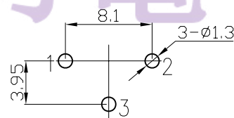
P.C.B LAYOUT (BOTTOM VIEW) Tolerance: ±0.05
