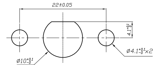
PANEL CUTOUT
