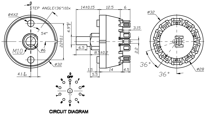
CIRCUIT DIAGRAM
