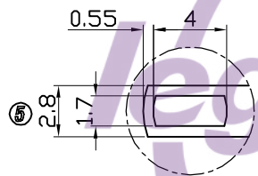
Solder Tab Type A
