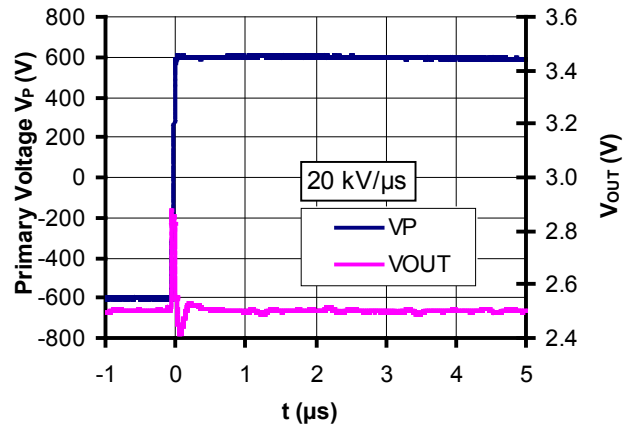
Figure 24: dv/dt
