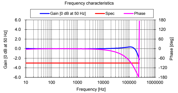
Figure 12: Frequency response
