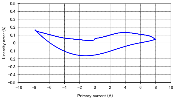
Figure 1: Linearity error
