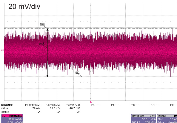
Figure 5: Output noise
