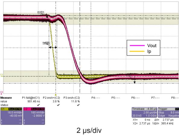
Figure 3: Step response
