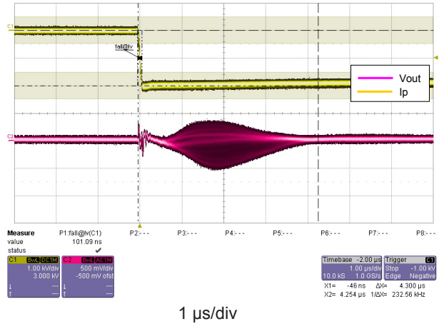
Figure 4: dv/dt
