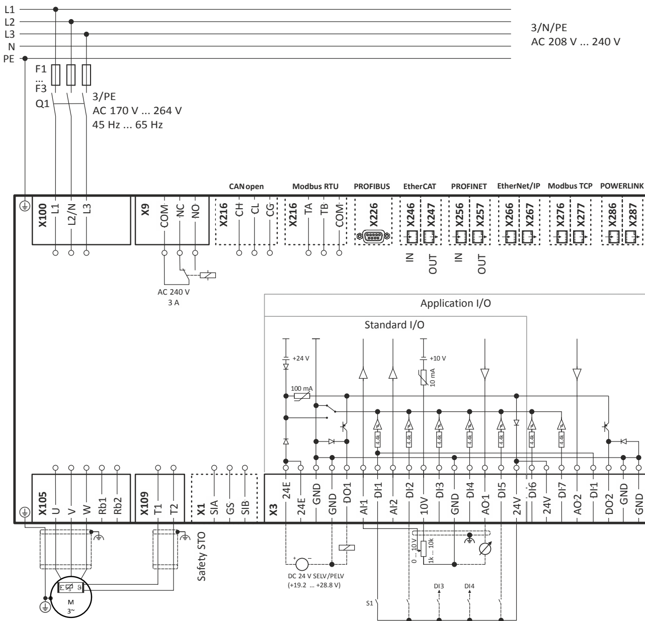
Fig. 7: Wiring example
