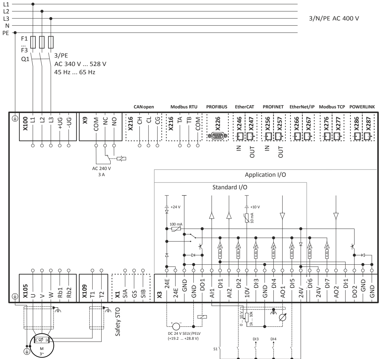
Fig. 8: Wiring example
