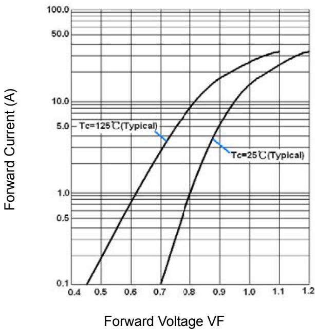
Fig.3 Forward Voltage
