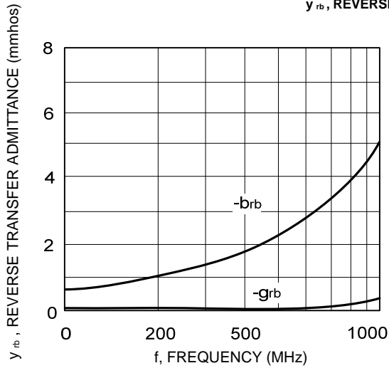
Figure 5. Rectangular Form
