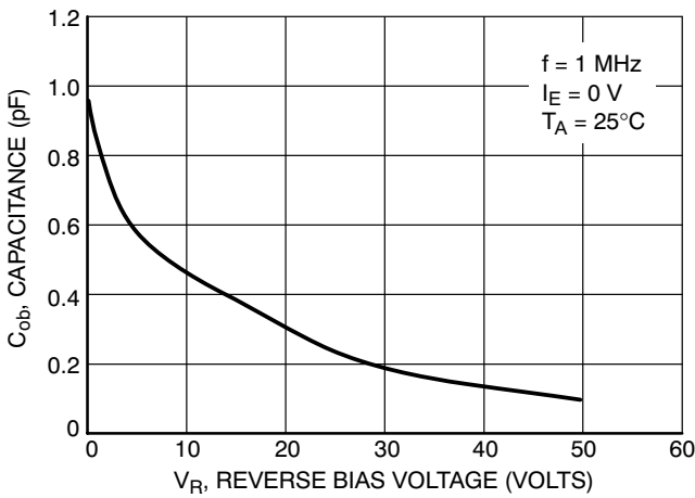
Figure 64. Output Capacitance
