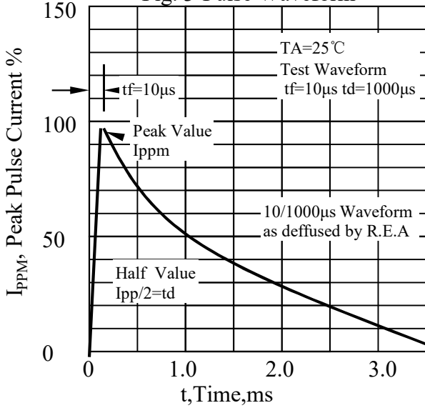
Fig. 3-Pulse Waveform
