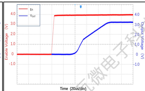
LW5430 ( V_{EN}=0V \rightarrow 4.0V , R_{OUT}=30\Omega )
