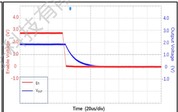
LW5418 ( V_{EN}=2.8V \rightarrow 0V , R_{OUT}=18 \Omega )
