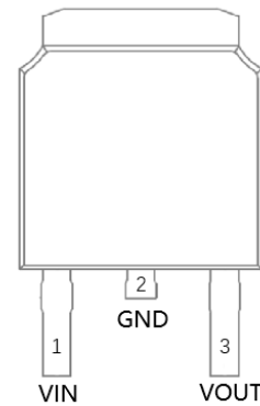
TO-252
