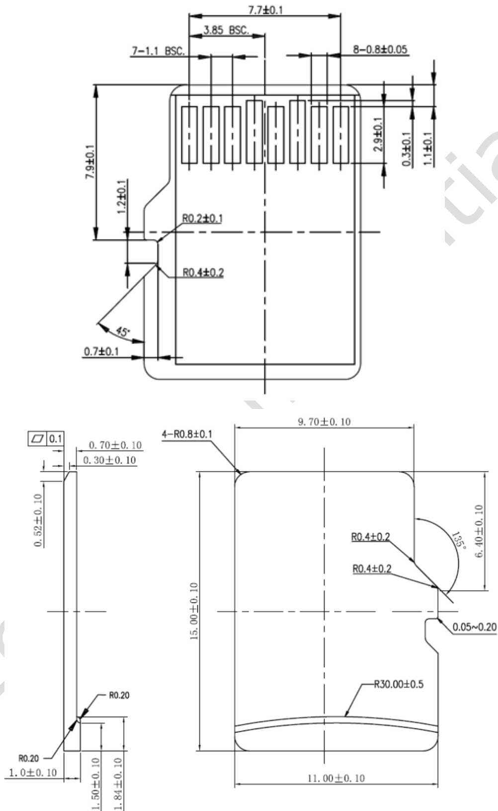
Figure 10: Dimension Drawing
