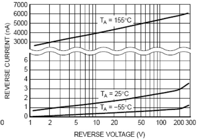
Figure 3. Reverse Leakage
