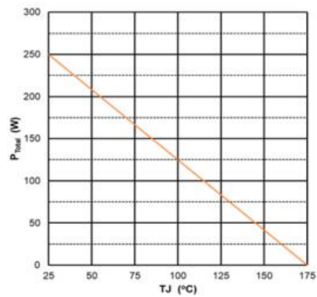
Figure 4. Power Derating
