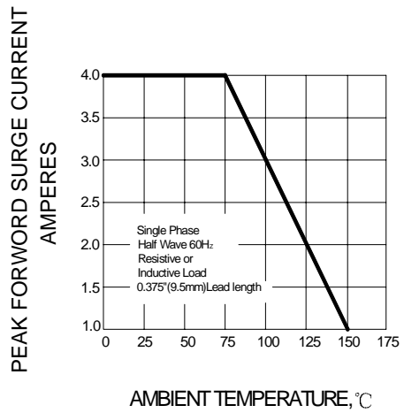
FIG.5 – FORWARD DERATING CURVE
