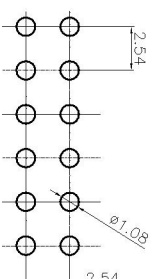
RECOMMENDED PCB LAYOUT TOLERANCE:±0.05
