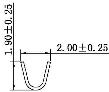
SEC B-B
