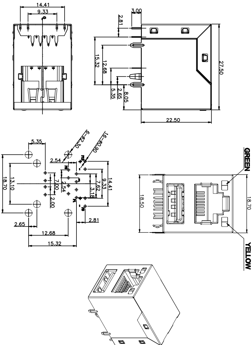
RECOMMENDED P.C.B LAYOUT TOP VIEW (COMPONENT SIDE)
