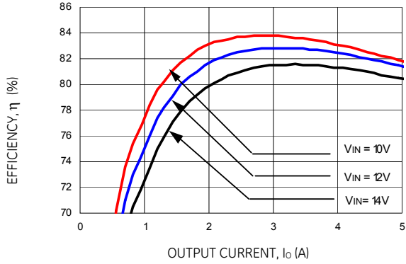
Figure 1. Converter Efficiency versus Output Current (Vout = 1.2Vdc).
