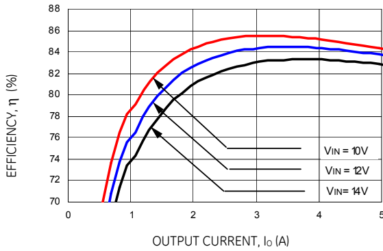
Figure 2. Converter Efficiency versus Output Current (Vout = 1.5Vdc).
