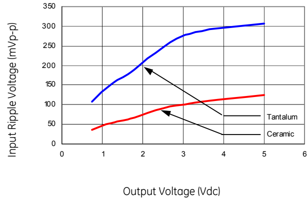
Figure 26. Input ripple voltage for various output with 2x47 µF tantalum capacitors and with 2x22 µF ceramic capacitors at the input (80% of I_{O,max} ).
