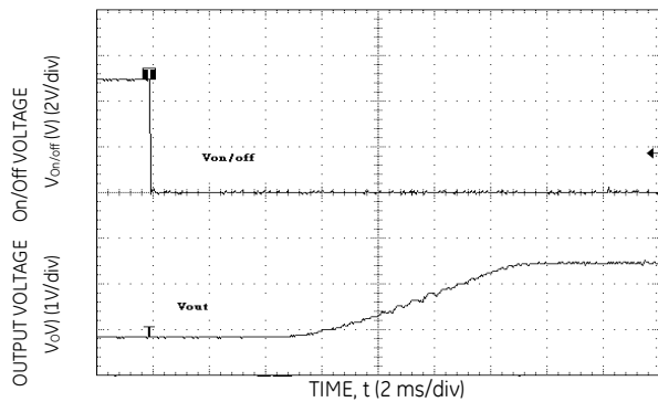
Figure 15. Typical Start-Up Using Remote On/Off with Low-ESR external capacitors ( 7 \times 150\mu\text{F} Polymer) ( V_{in} = 12\text{Vdc} , V_o = 3.3\text{Vdc} , I_o = 5.0\text{A} , C_o = 1050\mu\text{F} ).
