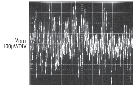
LT1761-5 10Hz to 100kHz Output Noise C BYP = 0pF
