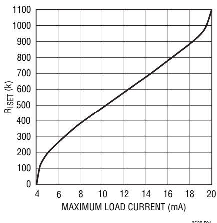
Figure 1. R_{ISET} Selection
