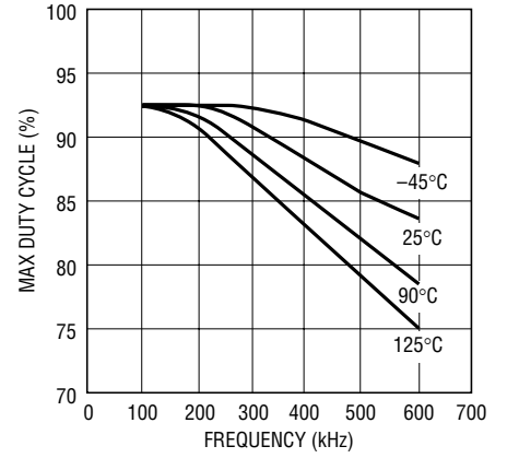
Max % DC vs Frequency and Temperature
