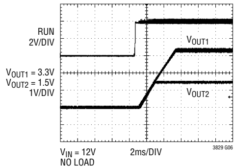
Coincident Tracking
