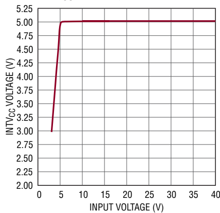
INT CC Line Regulation
