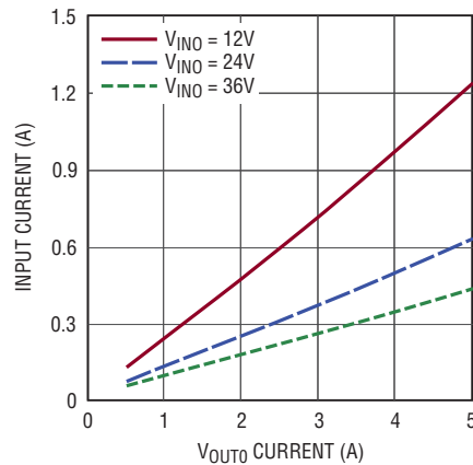
Input Current vs Output Current, V_{OUT0} = 2.5\text{V}
