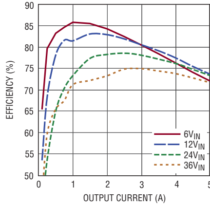
1.5V OUT Efficiency vs Output Current
